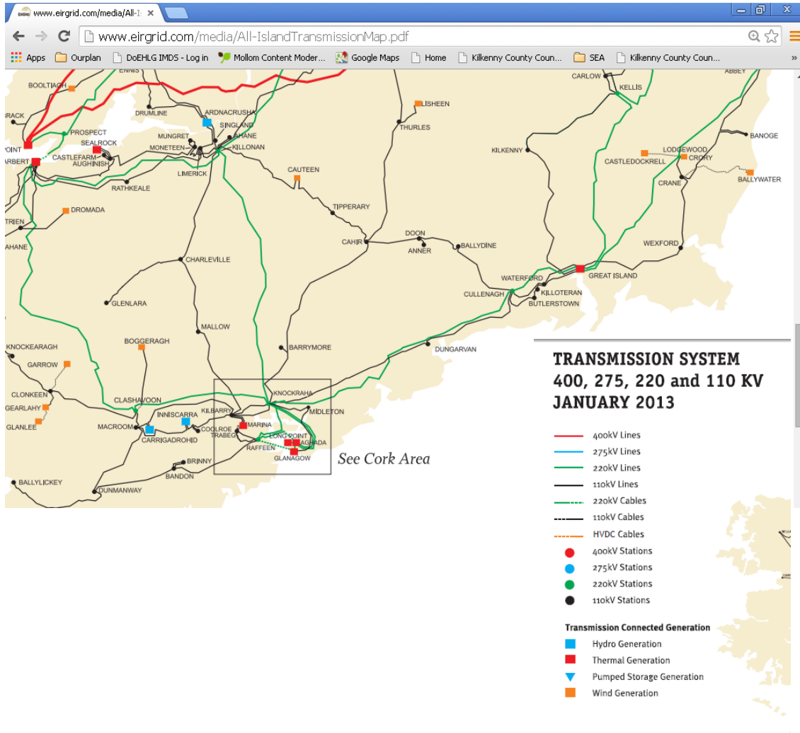
Figure 3.18 Transmission network in Plan area
